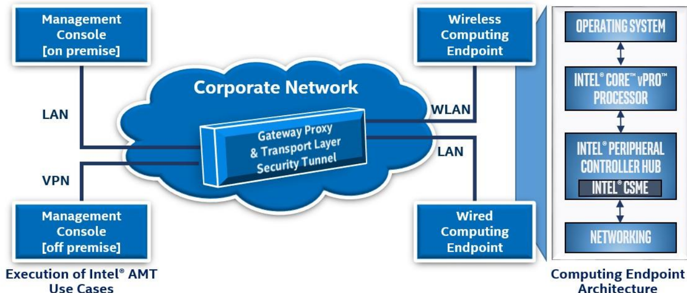
Figure 14: Typical Intel® AMT End-to-End Architecture described functions.
